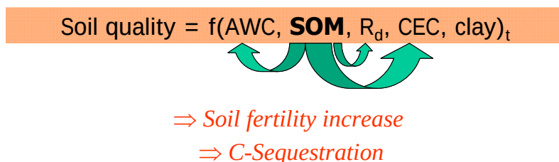
Fig. 1 Soil quality is a function (f) of available water holding capacity (AWC), soil organic matter level (SOM), root density ( R_d ), cation exchange capacity (CEC), clay content (clay) and time (t). The most important factor is SOM as it improves other variables such as AWC, R_d and CEC.
