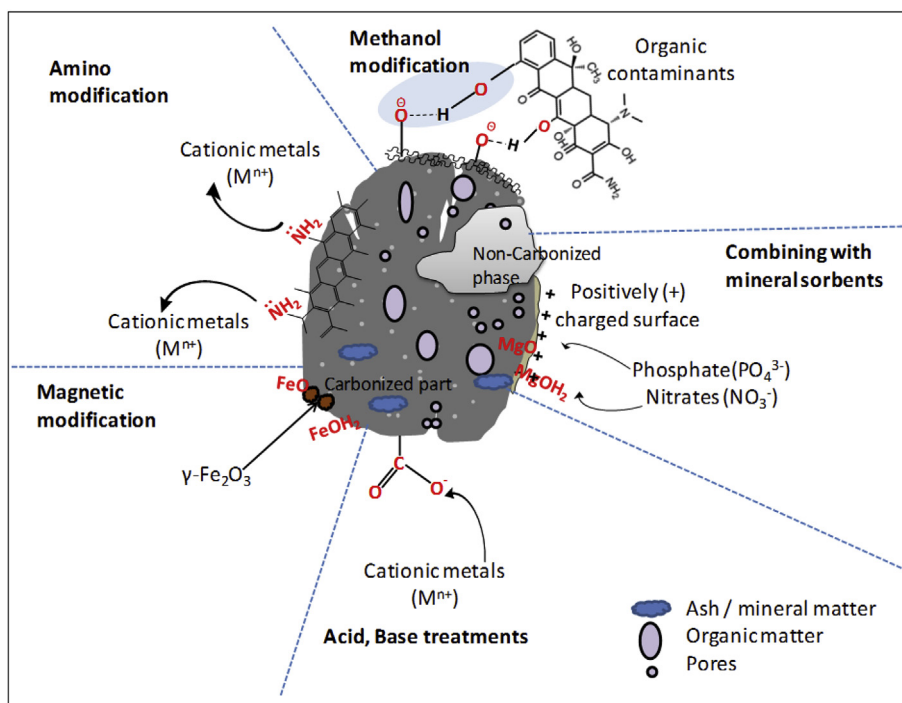
Fig. 1. Schematic diagram of biochar modifications.
